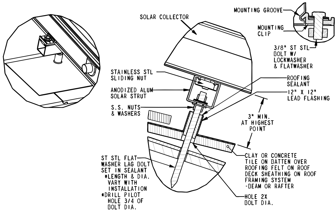
Figure 8 - Tile Roof Mounting
