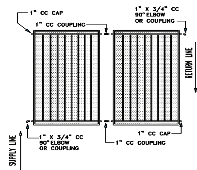
Figure 14 COLLECTOR PLUMBING - VERTICAL MOUNT
