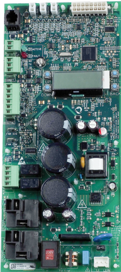
Control Board
