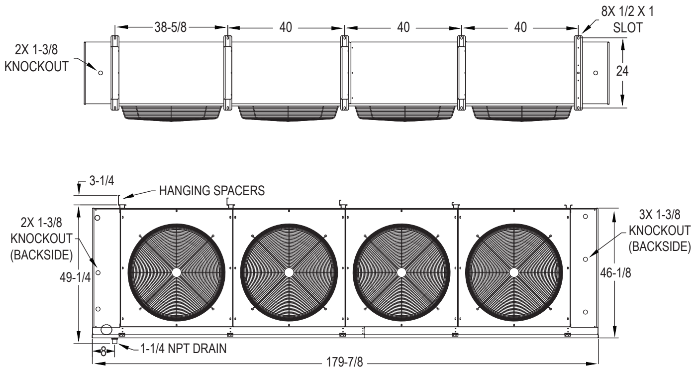
FIGURE 4 - FOUR FAN
