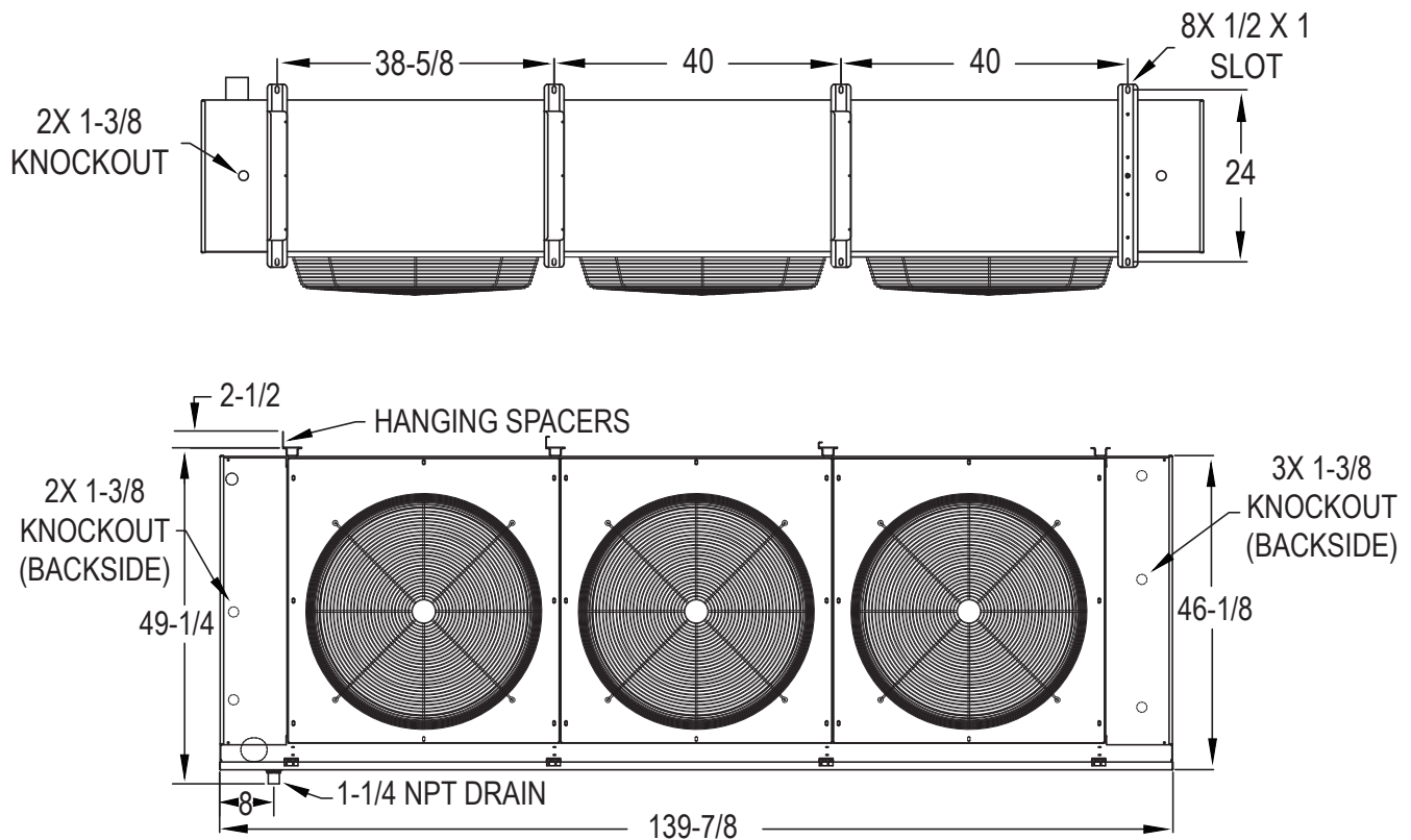
FIGURE 3 - THREE FAN
