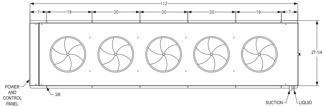
Figure 5 - Five Fan
