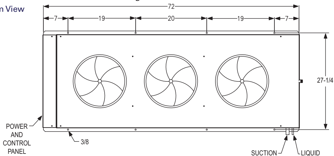
Figure 3 - Three Fan
