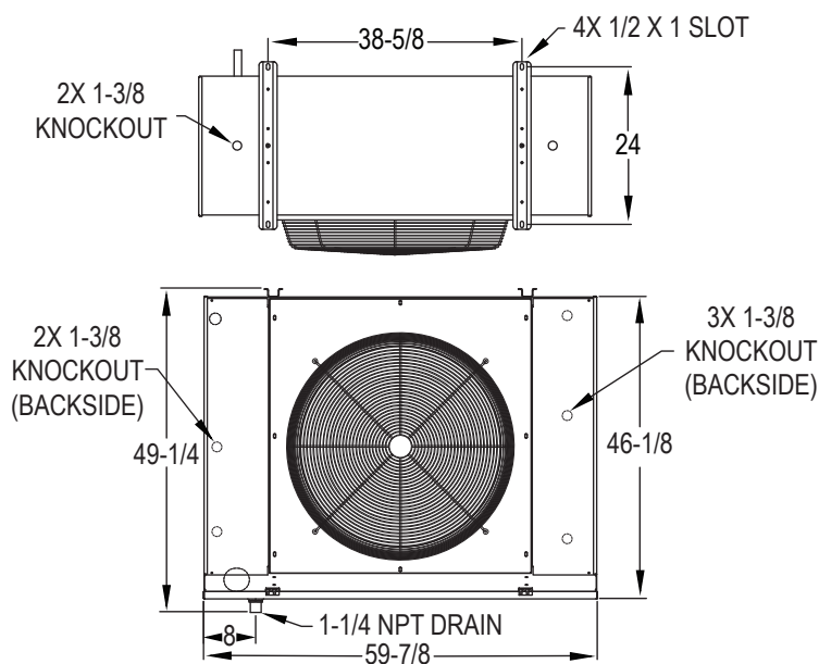
FIGURE 1 - SINGLE FAN
