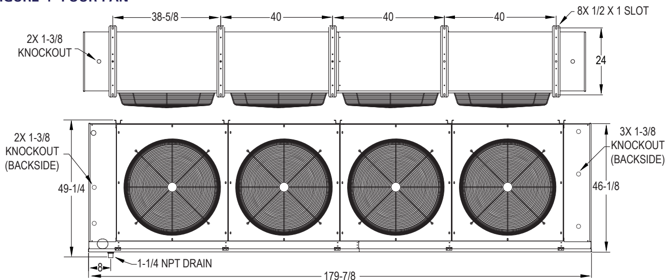
FIGURE 4- FOUR FAN
