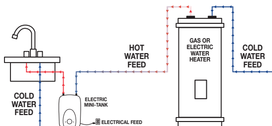
Standalone booster from central tank heating system
