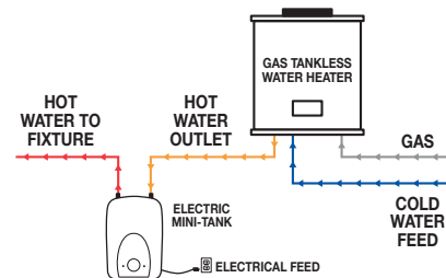
Cure for the "cold water sandwich" gas tankless
