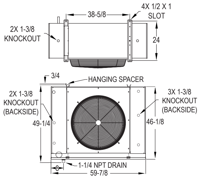
FIGURE 1 - SINGLE FAN
