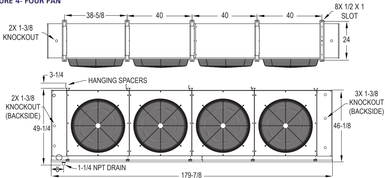
FIGURE 4- FOUR FAN
